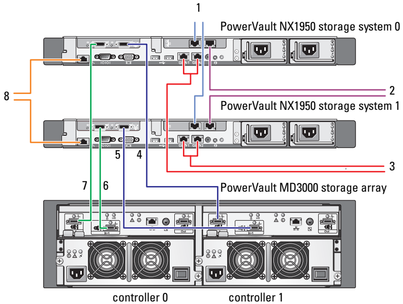
Figure 2-2. Two-Node Configuration
